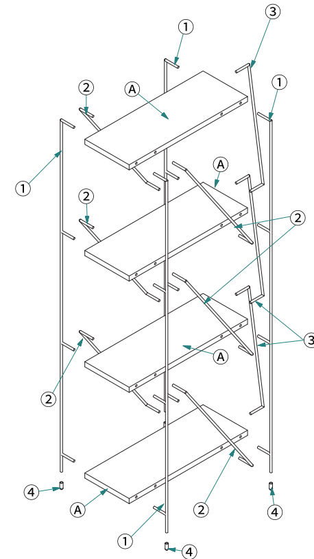
④ FOOT LEVELER PLASTIC - 4PCS
