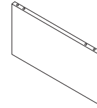
Ⓐ PANEL 15x200x400 - 4PCS
